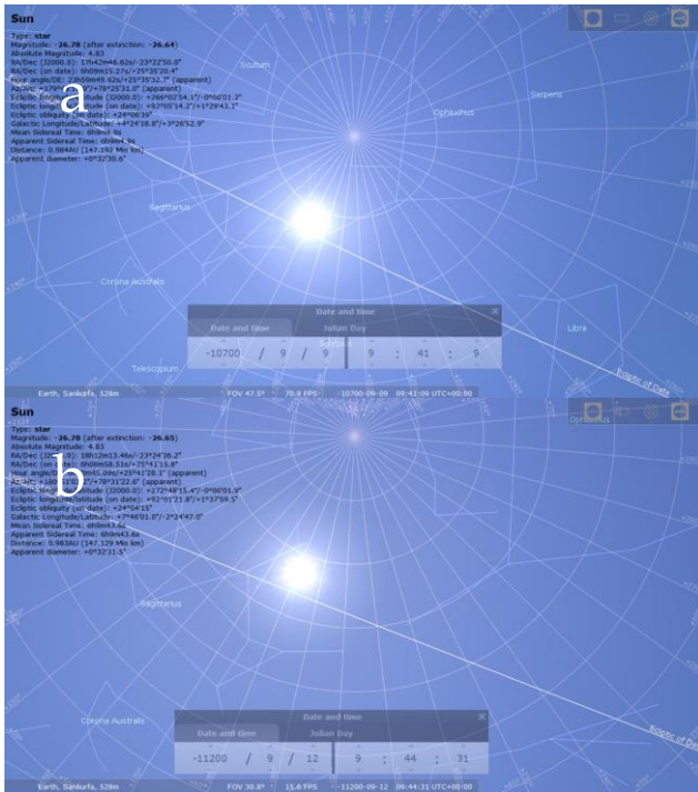
Figure 6. The sky at 10700 BC (a) and 11200 BC (b), as seen from Sanliurfa (near GT) as predicted by stellarium, from which an error estimate of the date stamp of 250 years is obtained.
